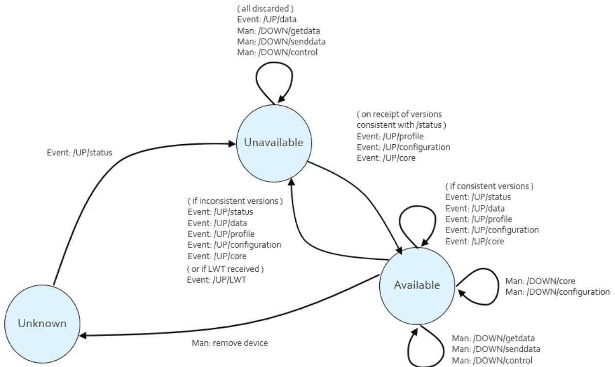
Figure 12 Connection state model
